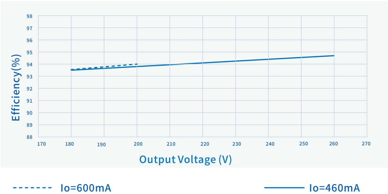
Efficiency Vs. O/P Voltage (Vin=347Vac)
